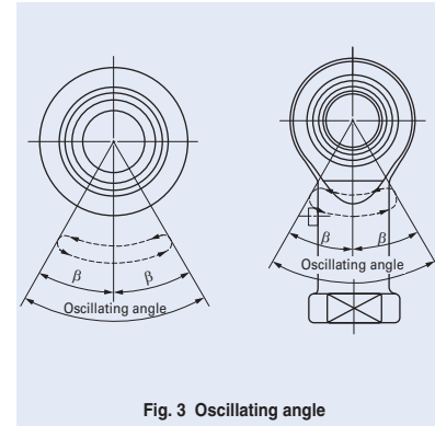
Fig. 3 Oscillating angle
