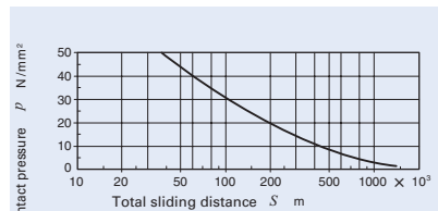
Fig. 6 Contact pressure and total sliding distance for maintenance-free type PILLOBALL Rod Ends
