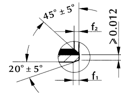
DETAIL Z
