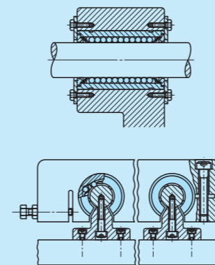
Fig. 6 Mounting example
